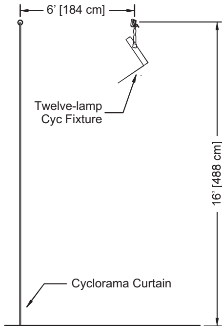
Partial Section
