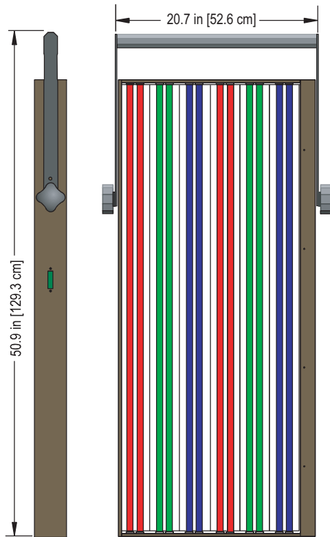
with vertical yoke
