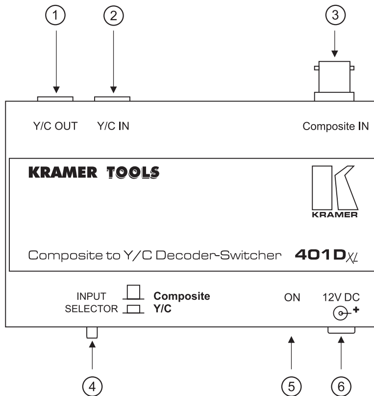
Figure 1: 401Dx/l Front Panel Features
