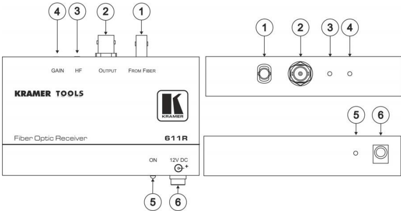
Figure 2: 611R Fiber Optic Receiver
