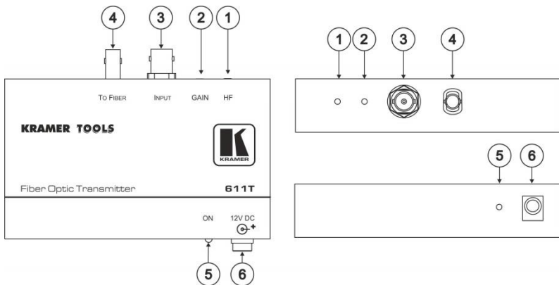
Figure 1: 611T Fiber Optic Transmitter
