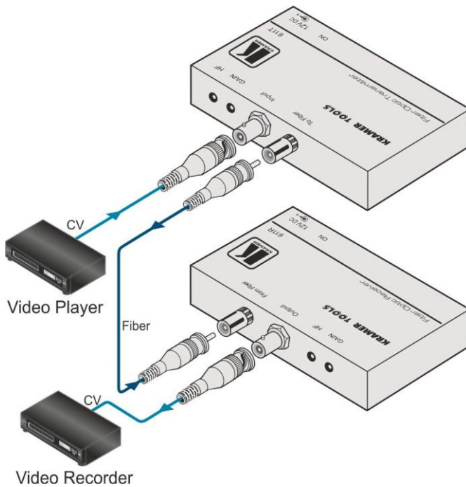
Figure 3: Connecting the 611T, 611R Fiber Optic Transmitter/Receiver
