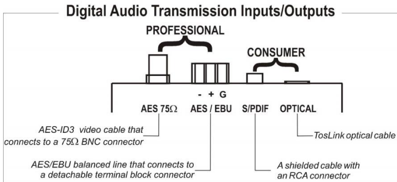
Figure 1: Professional and Consumer Inputs/Outputs on the 6410N / 6420N
