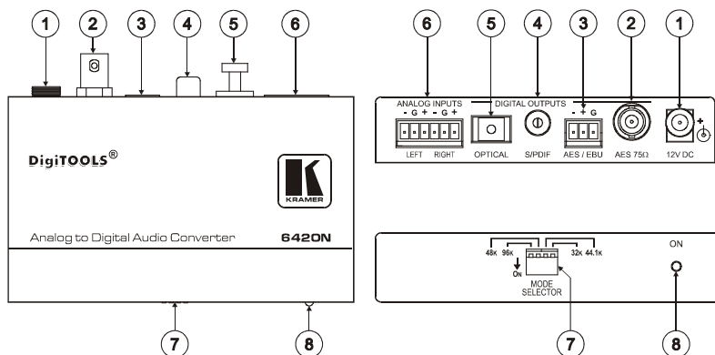
Figure 4: 6420N Analog to Digital Audio Converter
