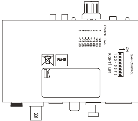
Figure 3: 6410N Digital to Analog Audio Converter Underside
