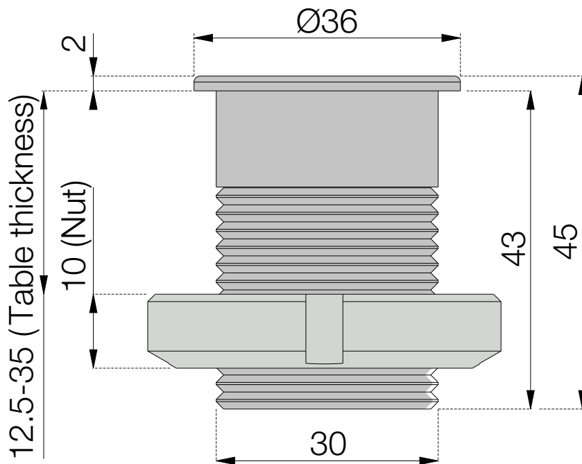
Front View (Bushing with nut)
