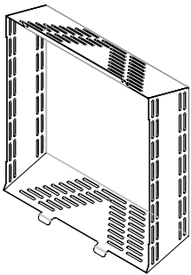
ACC-MS40-S ISOMETRIC VIEW
