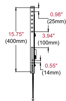
ADAPTOR BRACKET
