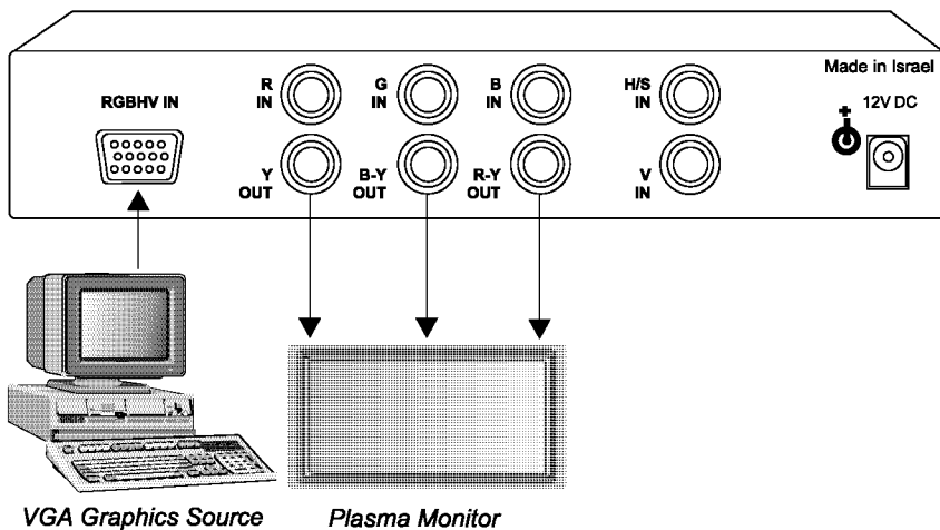
Figure 5: Converting from a VGA Graphics Source to a Plasma Monitor
