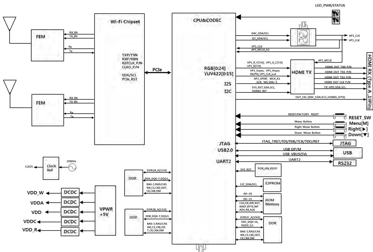
Receiver, HDWX-100Rx
