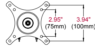
ADAPTER PLATE
