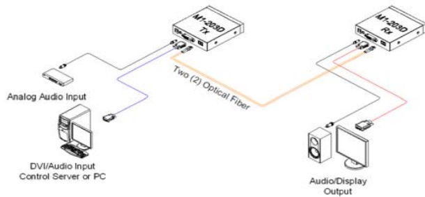
Figure 1 – Schematic Connection Diagram of Optical DVI/Audio Extension Modules
