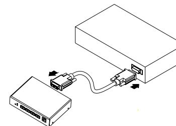
Figure 2 – Connection of DVI cable between Transmitter box and PC
