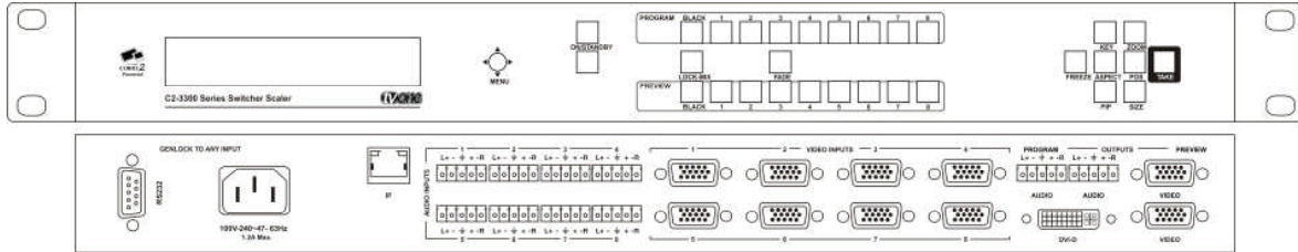
C2-3300 Series Front Panel and C2-3310 Rear Panel (with audio)
