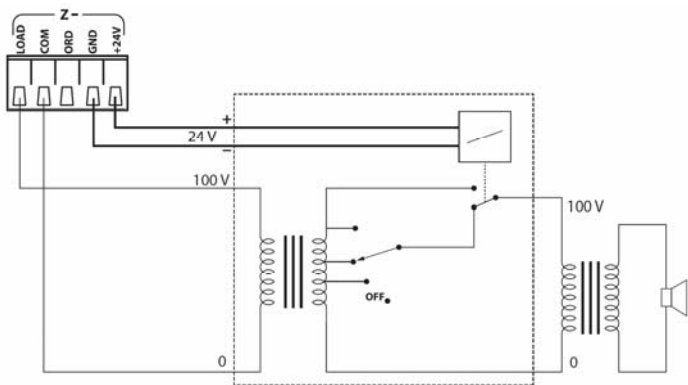
Scheme with 24 V Dc Bypass Relay
