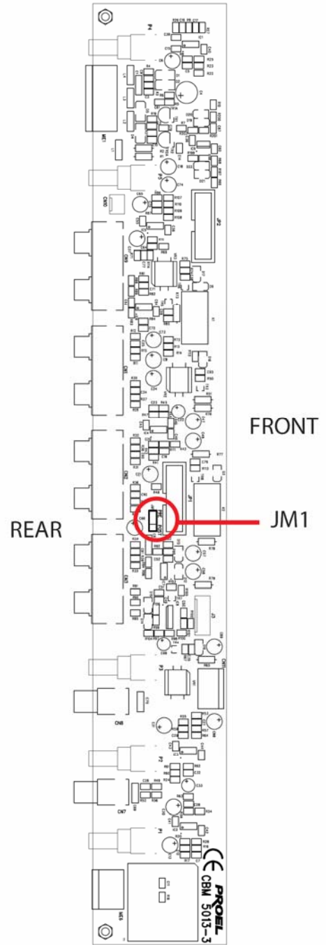
Rear Card inputs/outputs
