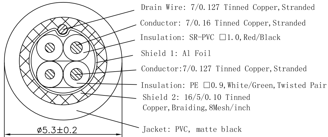
cable construction
