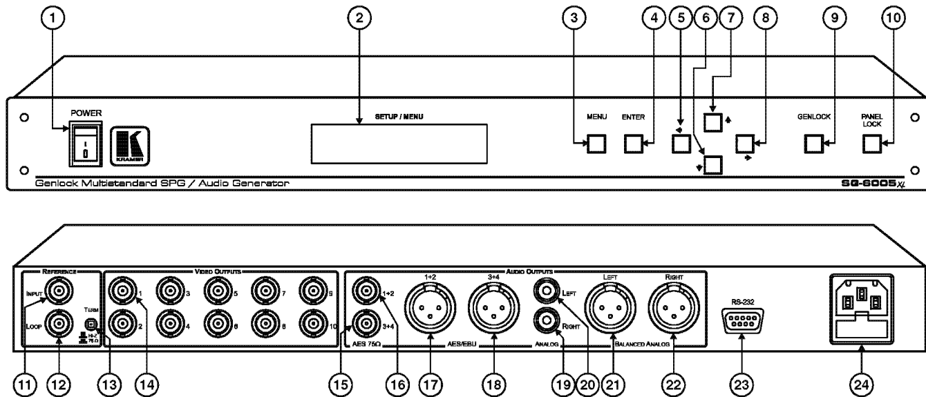
Figure 1: SG-6005xl Genlock Multistandard SPG / Audio Generator
