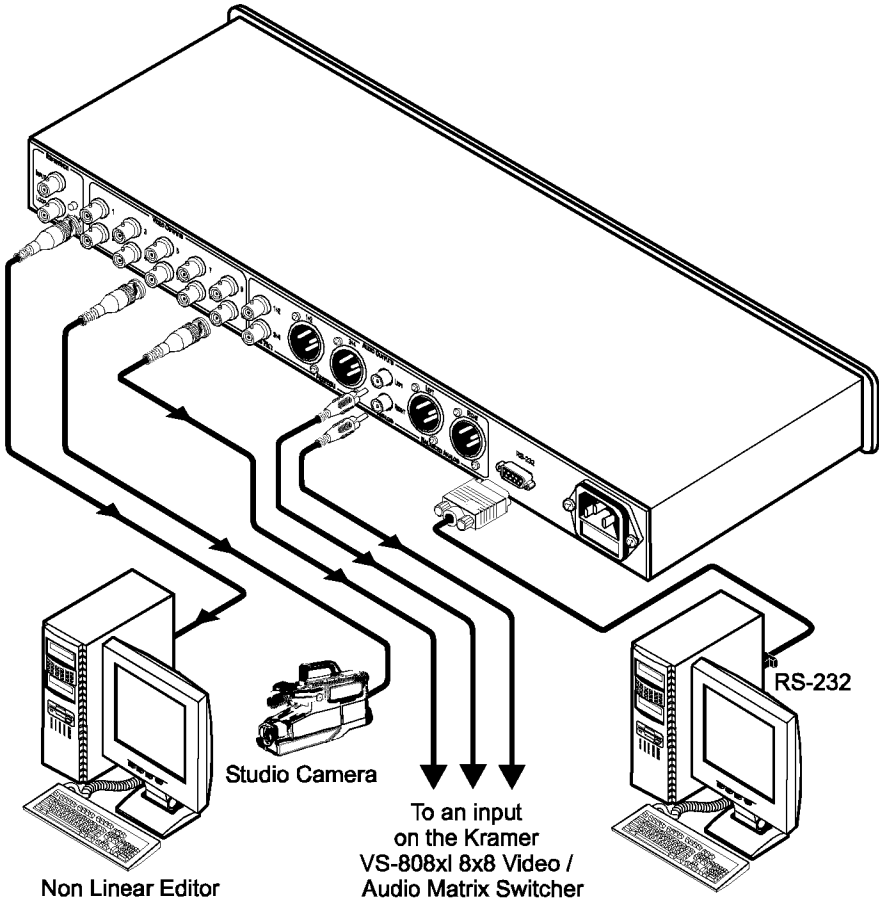
Figure 2: Connecting a SG-6005xl Genlock Multistandard SPG / Audio Generator
