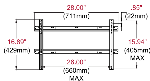
ADAPTOR DETAIL
