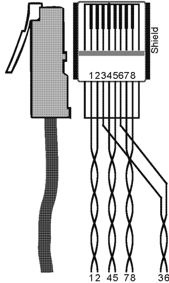
Figure 4: CAT 5 PINOUT
