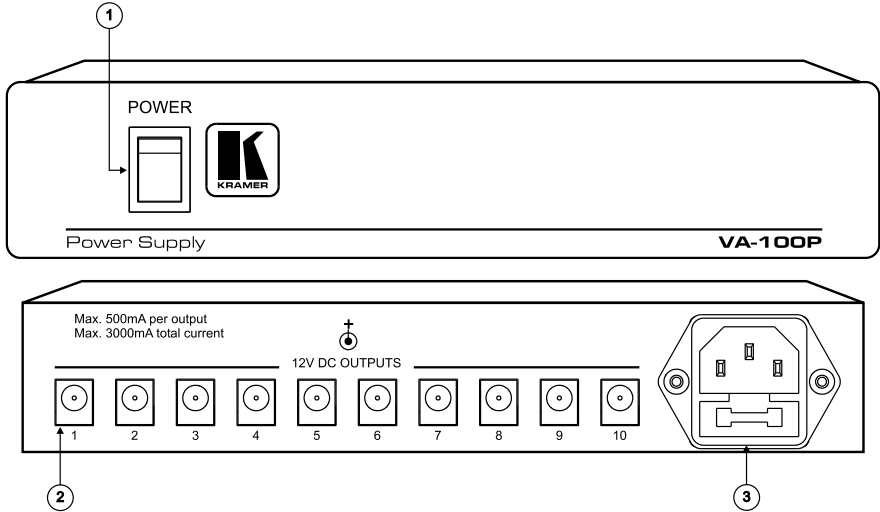
Figure 1: VA-100P Power Supply
