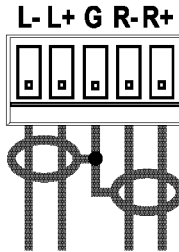
Figure 3: Connecting the Balanced Stereo Audio Input/Output
