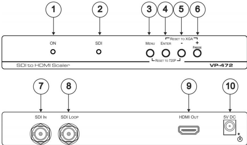
Figure 1: VP-472 SDI to HDMI Scaler
