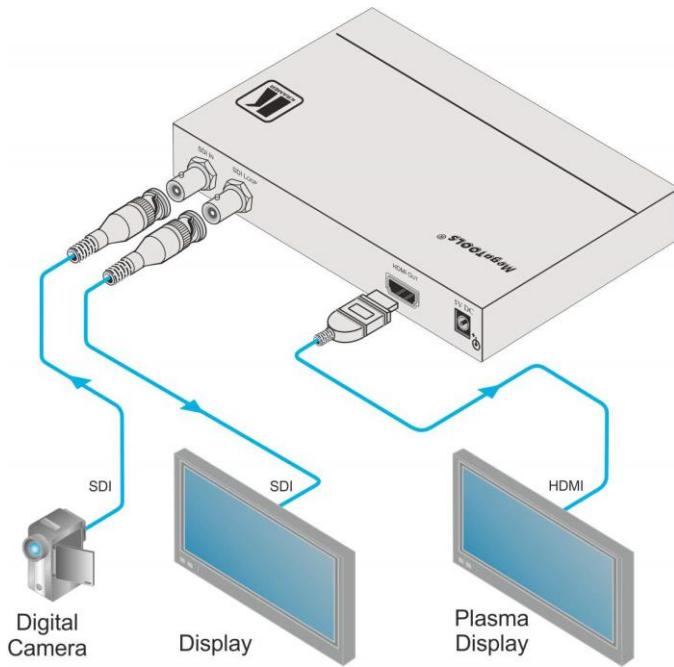
Figure 2: Connecting the VP-472 SDI to HDMI Scaler
