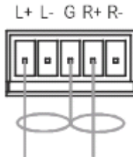
Figure 4: Connecting the Unbalanced Stereo Audio Output
