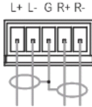
Figure 3: Connecting the Balanced Stereo Audio Output
