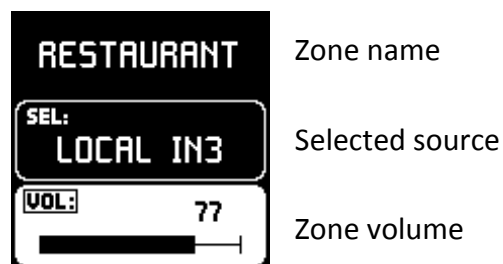
Figure 3: main screen
