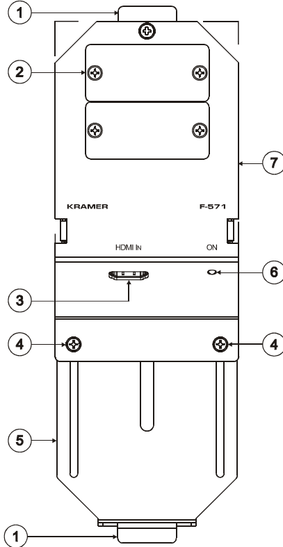
Figure 3: F-571 HDMI Line Transmitter Mounting Box
