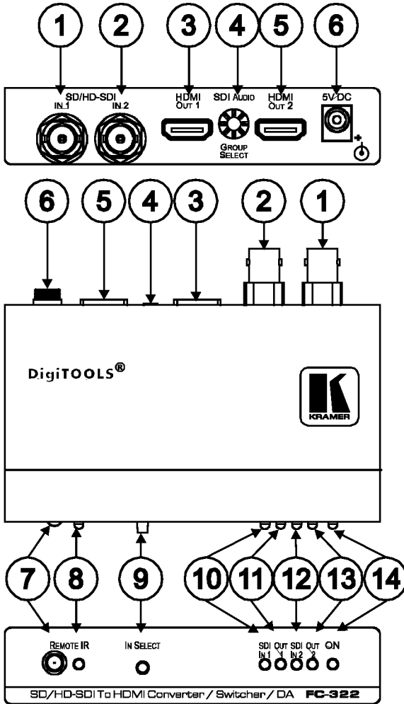
Figure 1: FC-322 SD/HD-SDI to HDMI Converter/Switcher/DA
