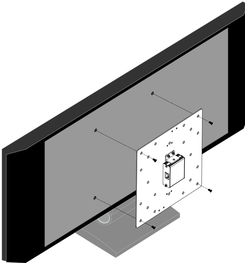
Figure 5: Attaching the MTH-1 to the Rear Side of the Display
