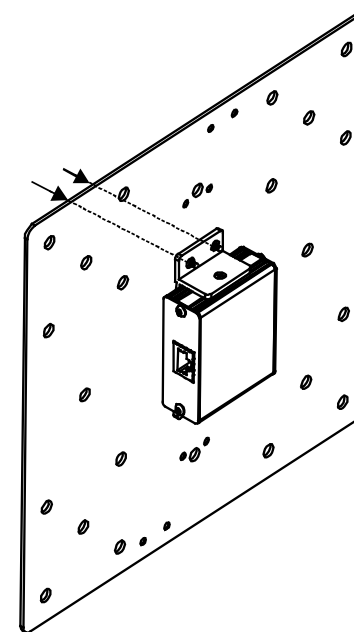
Figure 3: Attaching the TOOL to MTH-1
