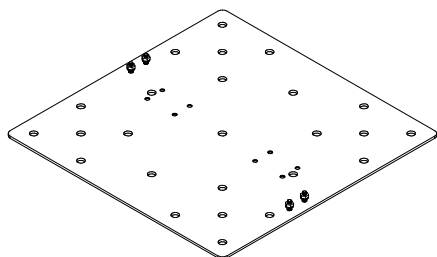
Figure 1: MTH-1 VESA Adapter Plate
