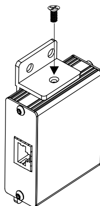
Figure 2: Installing the Brackets
