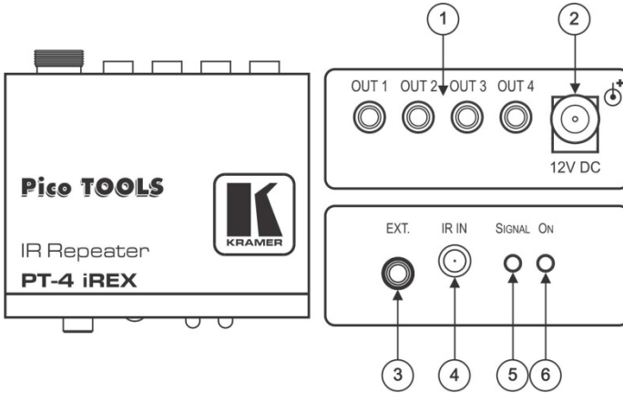
Figure 1: PT-4iREX IR Repeater
