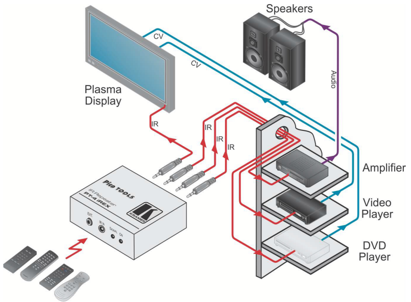
Figure 3: Connecting the PT-4iREX IR Repeater
