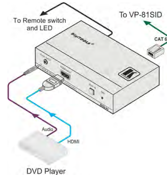
Figure 2: SID-H Wiring Connections
