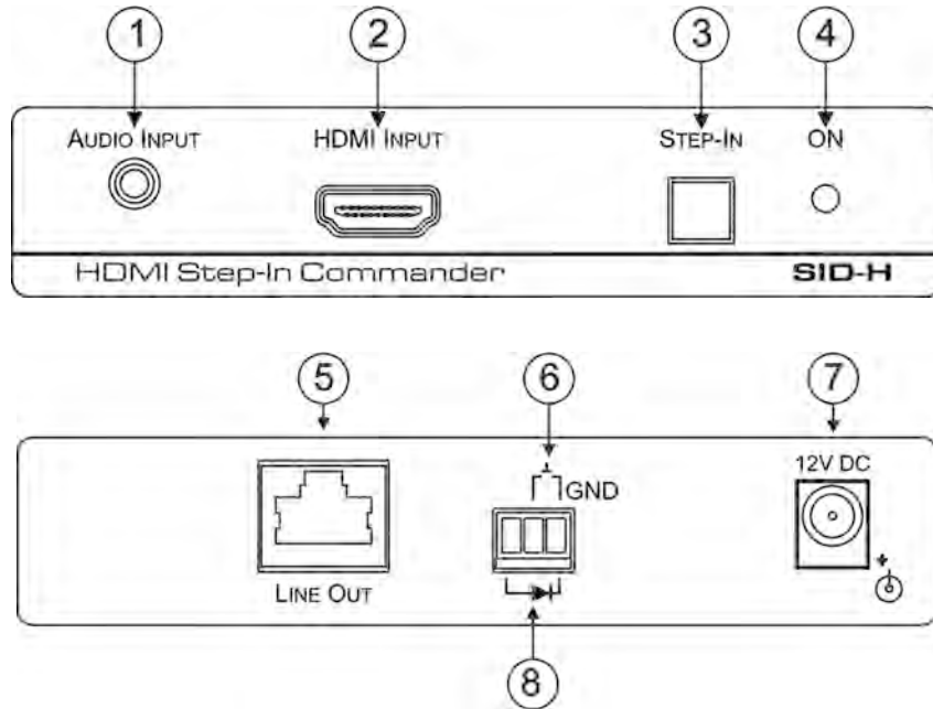
Figure 1: SID-H HDMI Step-In Commander Front and Rear Panel
