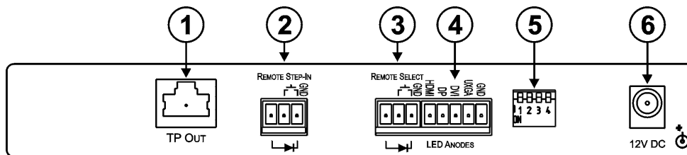
Figure 2: SID-X1 Step-In Commander Rear Panel
