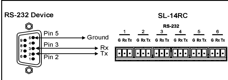
Figure 6: RS-232 Connection
