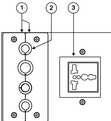
Figure 3: TBUS-9 Connecting Surface
