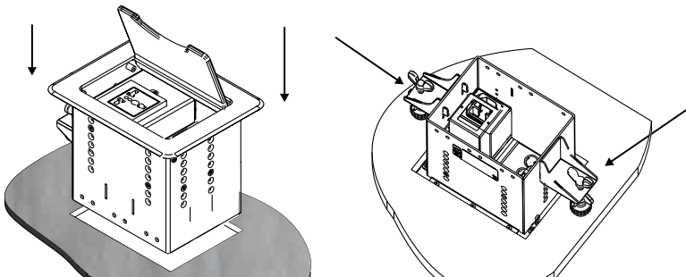
Figure 5: Installing TBUS-9
