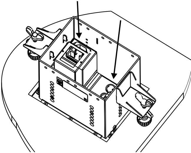
Figure 6: Connecting the Cables
