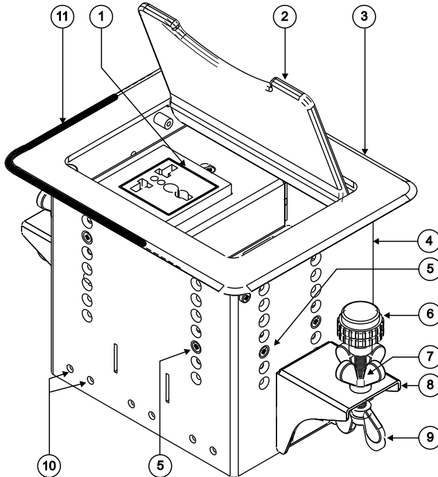
Figure 2: TBUS-9 Table Connection Bus (Top View)
