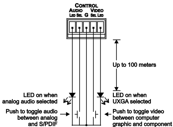
Figure 4: The TP-45EDID Remote Control Connection
