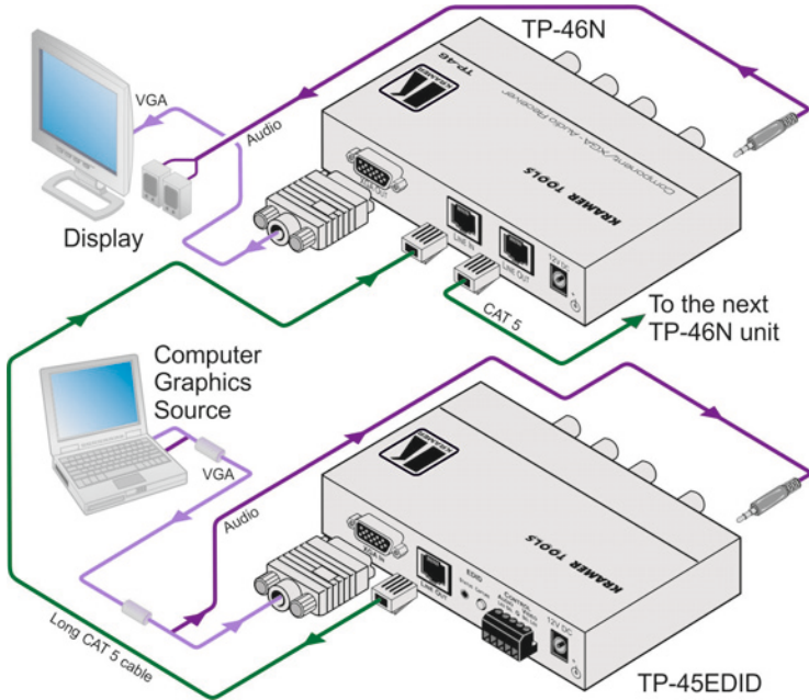
Figure 2: Component/XGA – Audio Distribution System, XGA Mode
