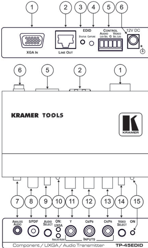
Figure 1: TP-45EDID Component/UXGA/Audio Transmitter
