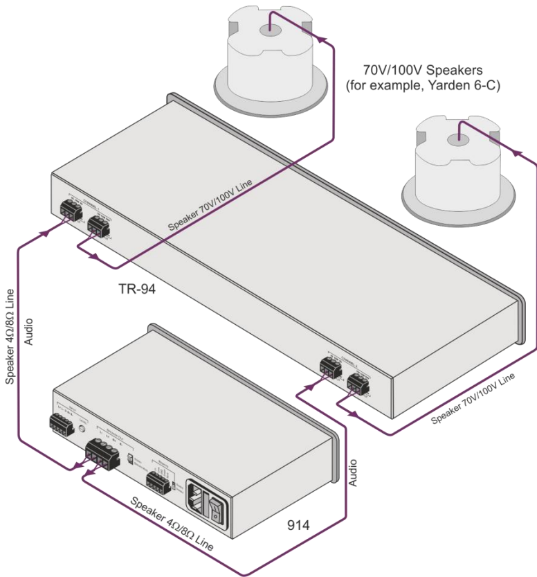
Figure 4: Connecting the TR-94 2x200W Audio Transformer
