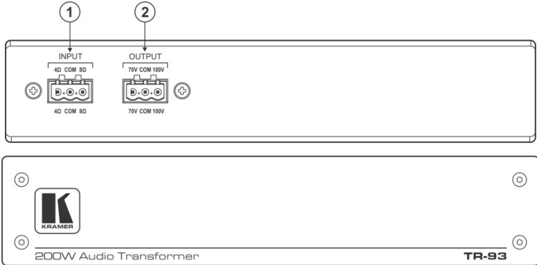
Figure 1: TR-93 200W Audio Transformer
