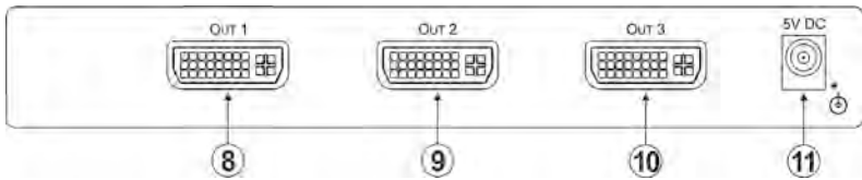
Figure 2: VM-400HDCP 1:4 DVI Distributor Rear Panel
