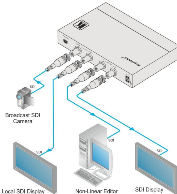
Figure 2: Connecting the VP-470 SD / 3G HD-SDI Scaler
