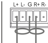
Unbalanced stereo audio connection
