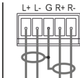
Balanced stereo audio connection
