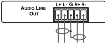
Figure 5: Connecting the Balanced Stereo Audio Output
