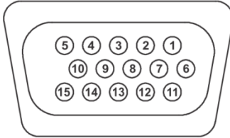
Figure 4: UNIV 15-pin HD Connector Pinout
