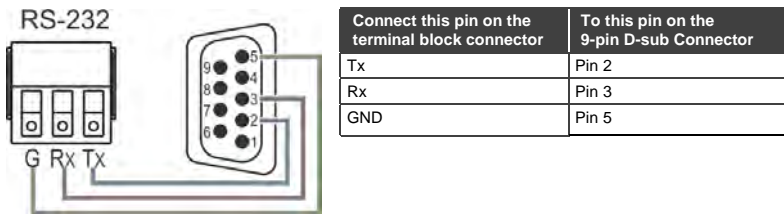
Figure 5: RS-232 Pinout
