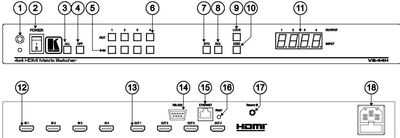
Figure 1: VS-44H 4 x 4 HDMI Matrix Switcher Front and Rear Views
