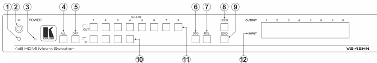
Figure 1: VS-48HN 4x8 HDMI Matrix Switcher Front Panel
