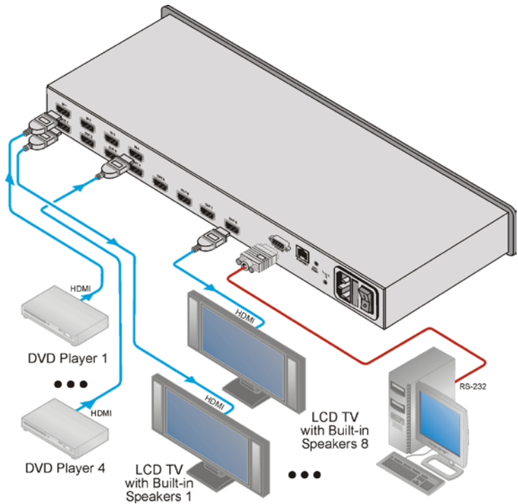
Figure 3: Connecting the VS-48HN 4x8 HDMI Matrix Switcher
