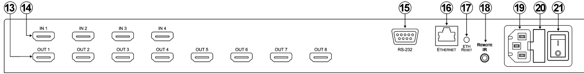
Figure 2: VS-48HN 4x8 HDMI Matrix Switcher Rear Panel
